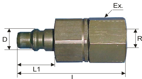
NIPLE ROSCA INTERIOR METRICA
